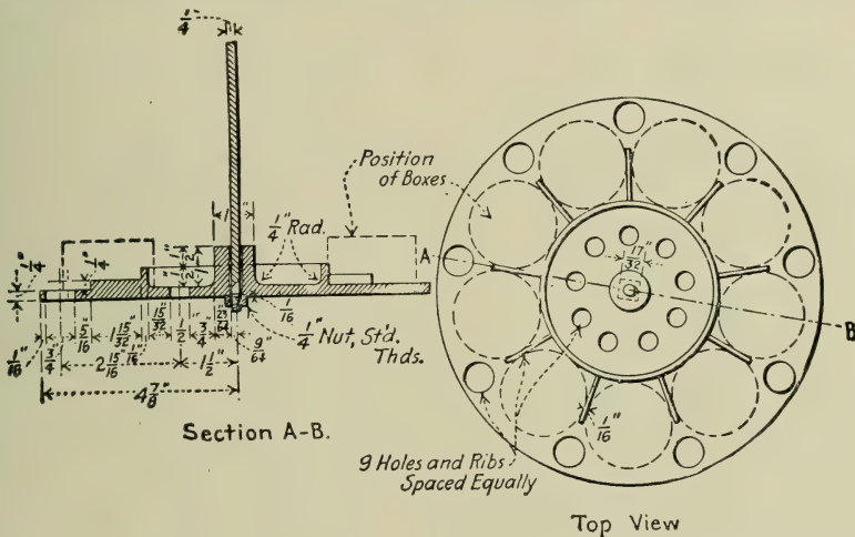
Fig. 180.—Shelf for Volatility Oven.
